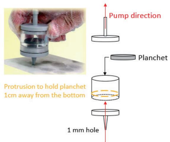
Fig.3 Structure of the impactor. The impactor is connected with vacuum pump via tube and filter trap. The range of grain size of particles can be controlled by vacuum flow rate.
