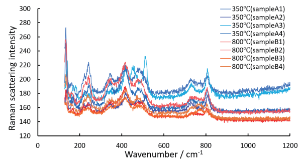
Fig.17 Raman peaks of sample A and B. \text{U}_3\text{O}_8 shows raman peaks at 241\text{ cm}^{-1} , 348\text{ cm}^{-1} , 412\text{ cm}^{-1} , 493\text{ cm}^{-1} , 731\text{ cm}^{-1} , 806\text{ cm}^{-1} . Raman peak of sample A3 indicates sample A including uranium oxides other than \text{U}_3\text{O}_8 .
